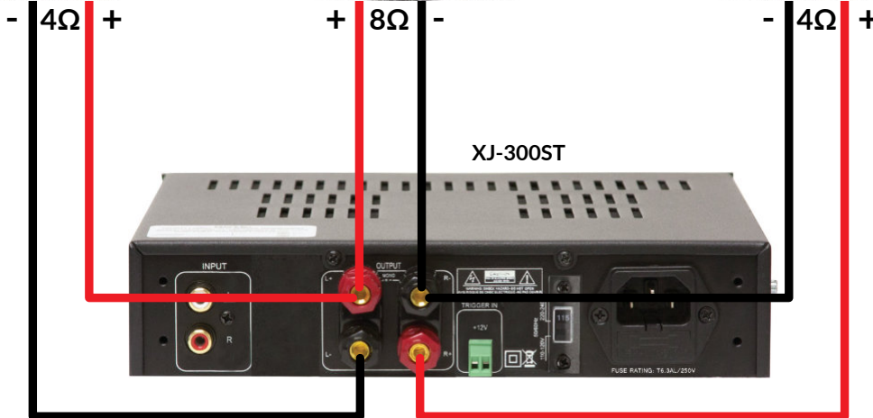
TRI-MODE WIRING CONFIGURATION WITH XJ-300ST
