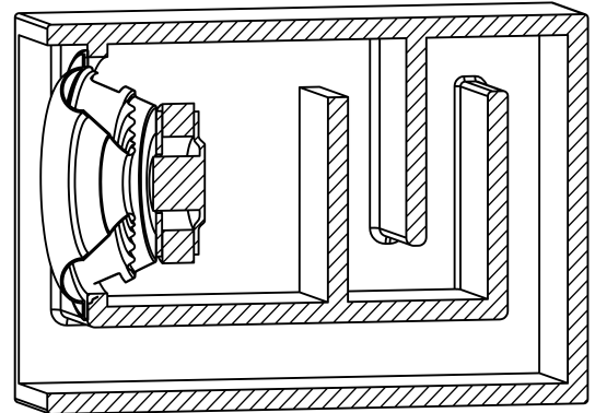
FF6.5 Transmission Line Design
